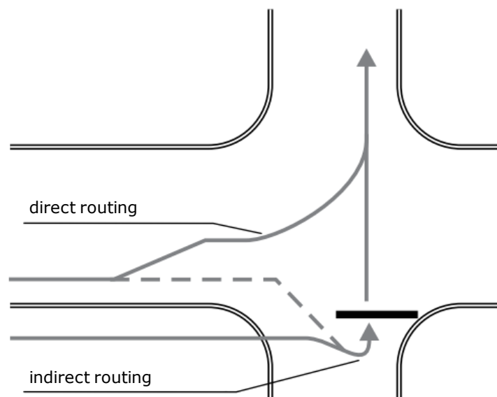
Figure 7 – Direct and indirect routing of left-turning bicycles at intersections (Source: FGSV, 2010b)
