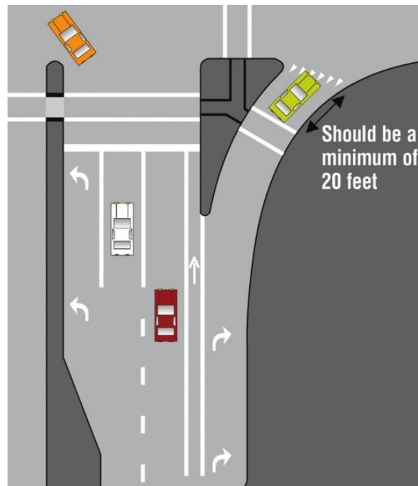
Figure 8 – Pedestrian crossing at channelised right-turn lane (Source: FHWA, 2014a)
