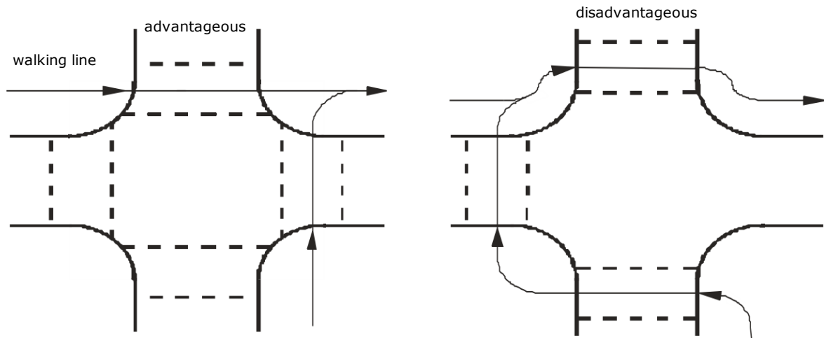
Figure 6 – Advantageous and disadvantageous location of crossings at signalised intersections (Source: FGSV, 2002)
